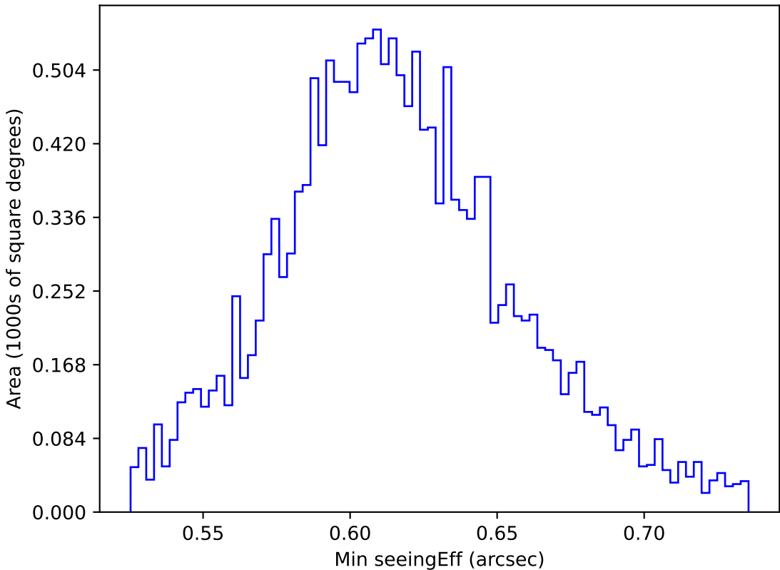
too_elab_r32_d2_ugrizy_v3.4_10yrs WFD z band: Min seeingEff
