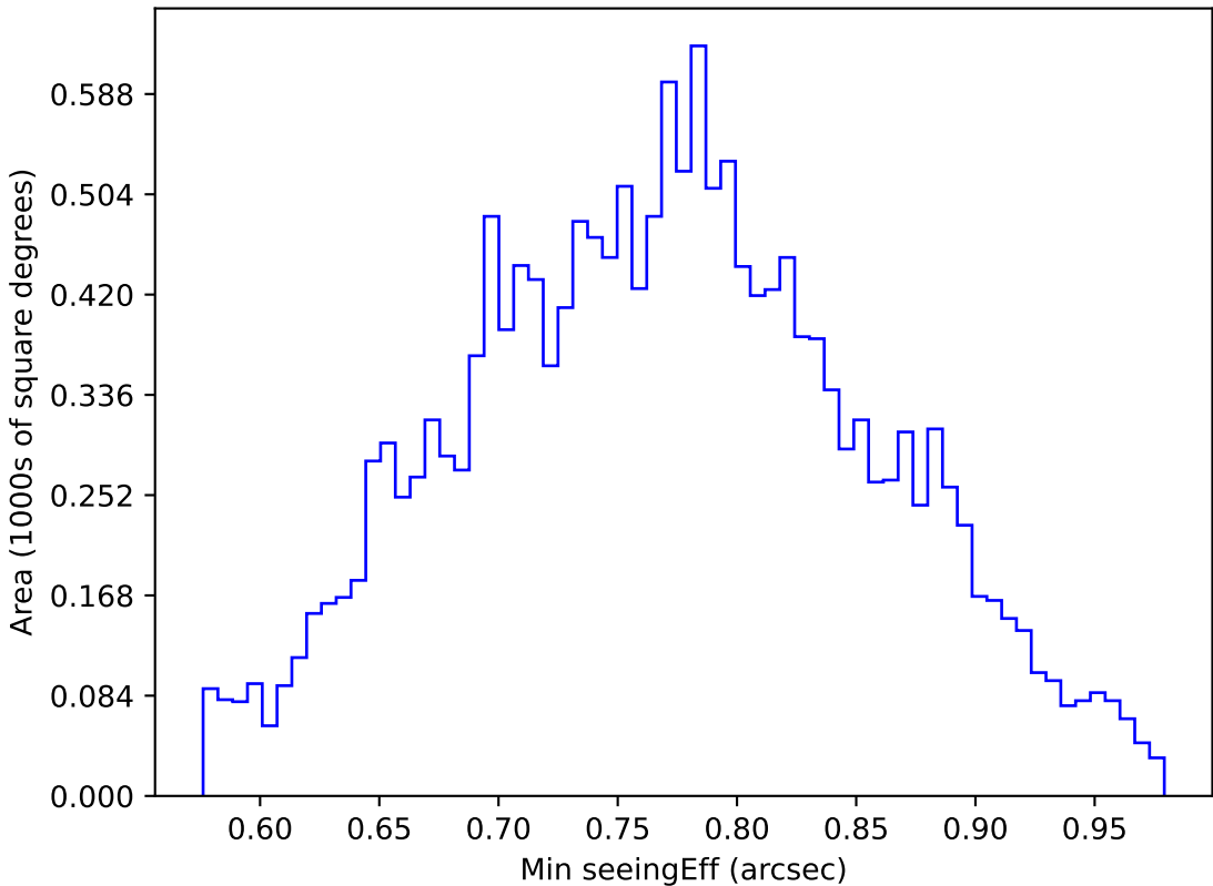
too_elab_r32_d2_ugrizy_v3.4_10yrs WFD u band: Min seeingEff
