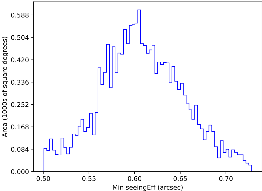
too_elab_r32_d2_ugrizy_v3.4_10yrs WFD r band: Min seeingEff
