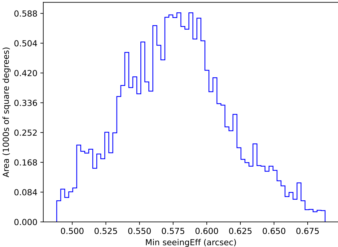
too_elab_r32_d2_ugrizy_v3.4_10yrs WFD all bands: Min seeingEff
