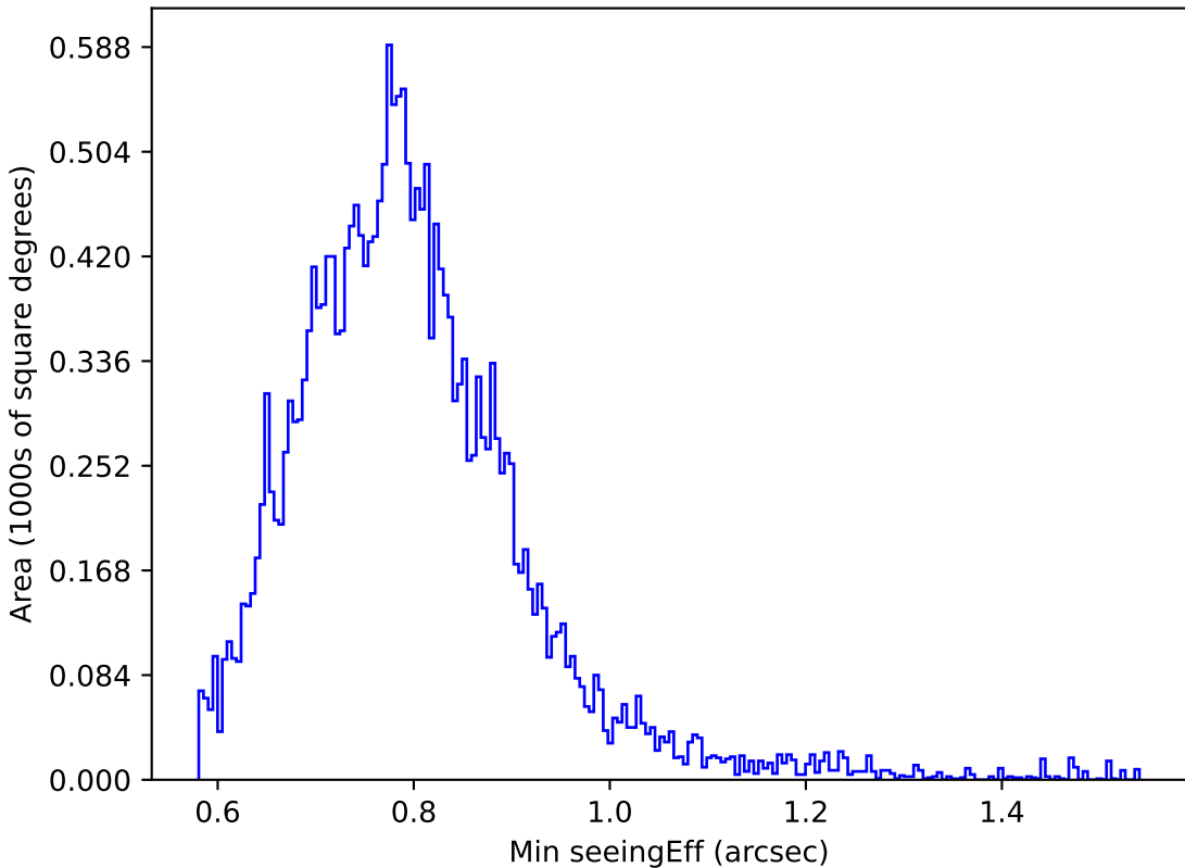
too_elab_r32_d2_ugrizy_v3.4_10yrs All sky u band: Min seeingEff
