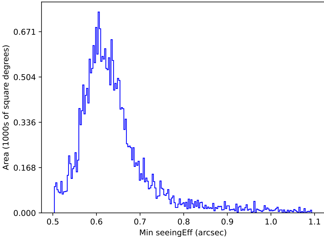
too_elab_r32_d2_ugrizy_v3.4_10yrs All sky r band: Min seeingEff
