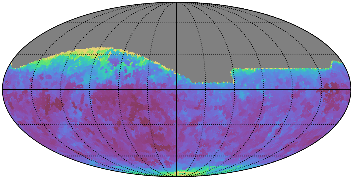
too_elab_r32_d2_ugrizy_v3.4_10yrs All sky i band: Min seeingEff
