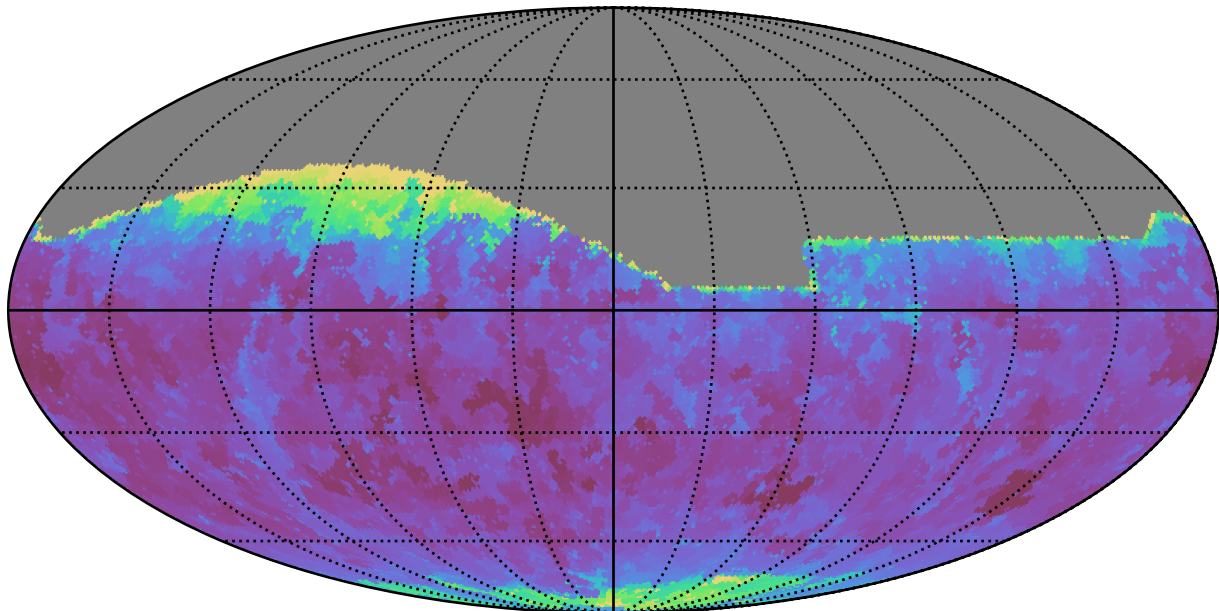
too_elab_r32_d2_ugrizy_v3.4_10yrs All sky g band: Min seeingEff
