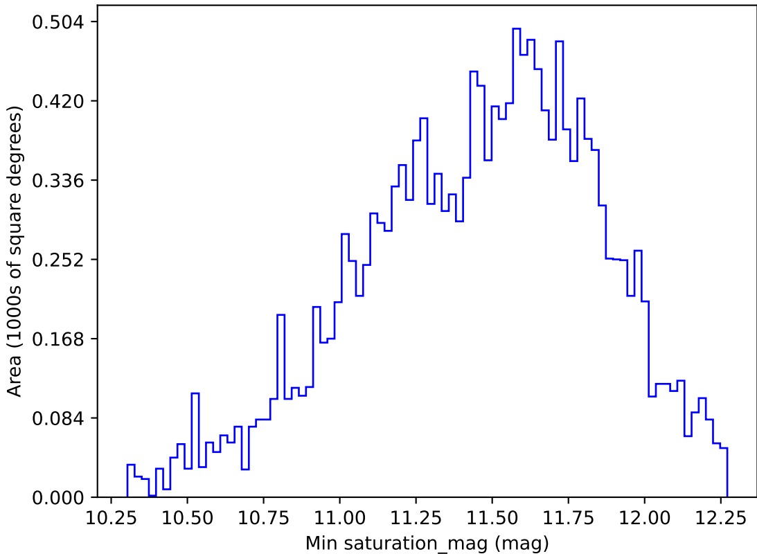
too_elab_r32_d2_ugrizy_v3.4_10yrs WFD u band: Min saturation_mag
