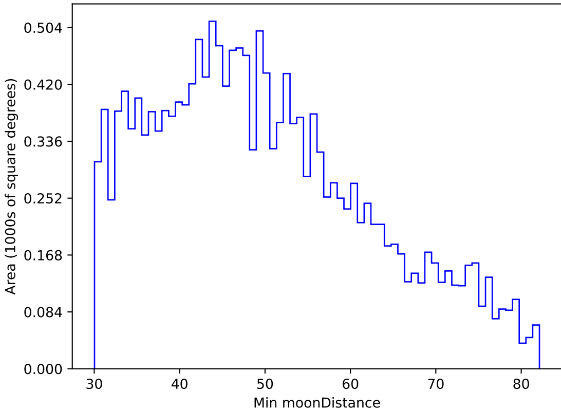
too_elab_r32_d2_ugrizy_v3.4_10yrs WFD u band: Min moonDistance
