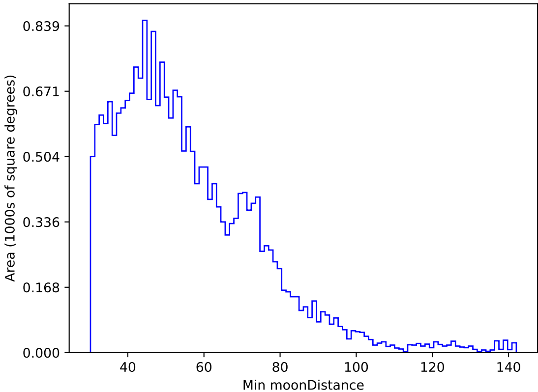
too_elab_r32_d2_ugrizy_v3.4_10yrs All sky u band: Min moonDistance
