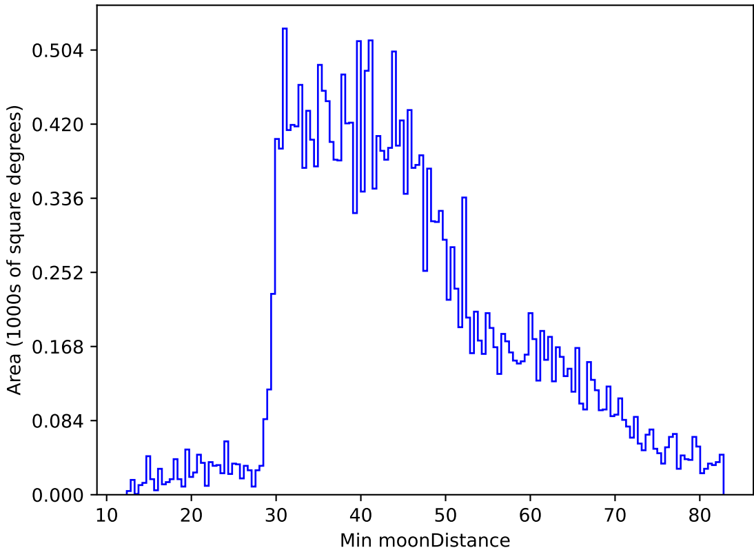
too_elab_r32_d2_ugrizy_v3.4_10yrs All sky g band: Min moonDistance
