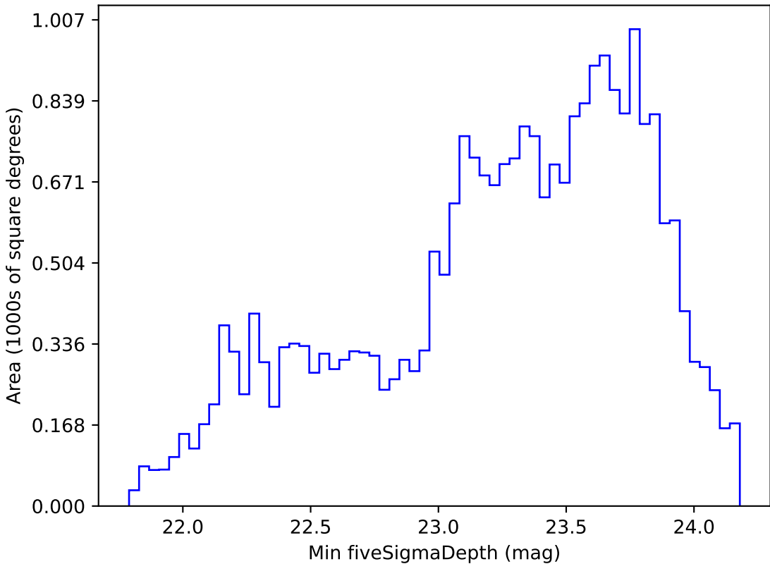
too_elab_r32_d2_ugrizy_v3.4_10yrs Yr 1 r band: Min fiveSigmaDepth
