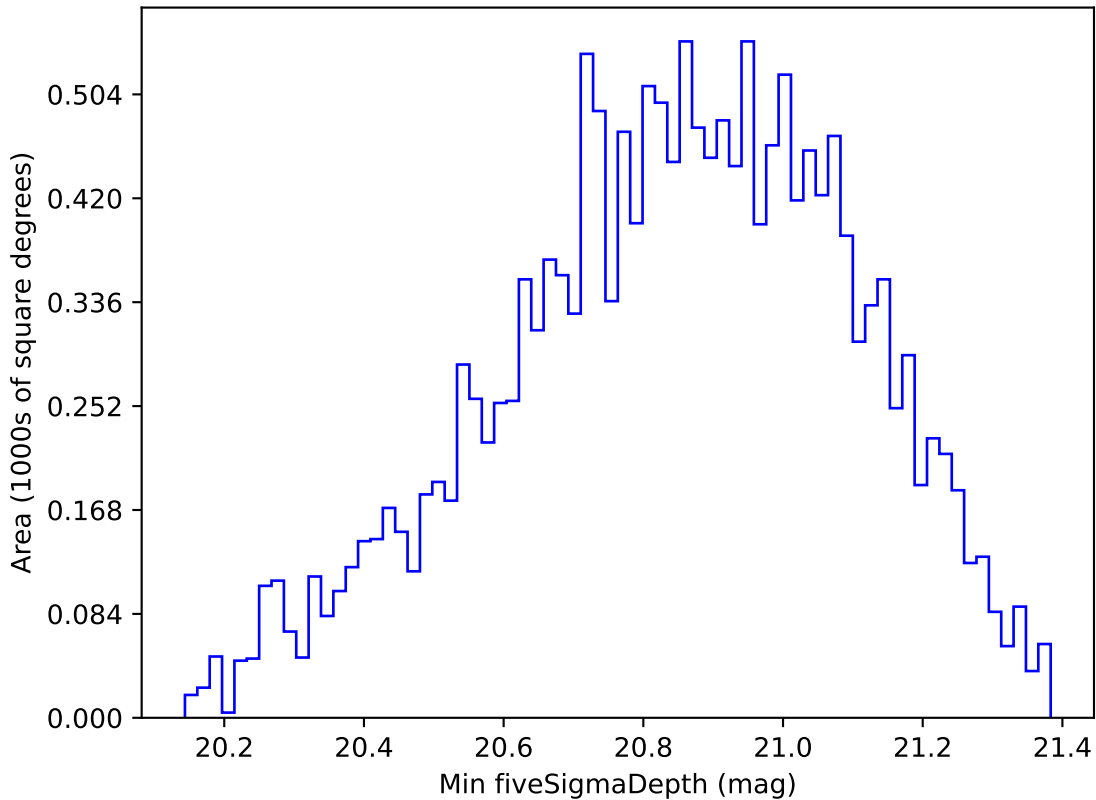
too_elab_r32_d2_ugrizy_v3.4_10yrs WFD y band: Min fiveSigmaDepth
