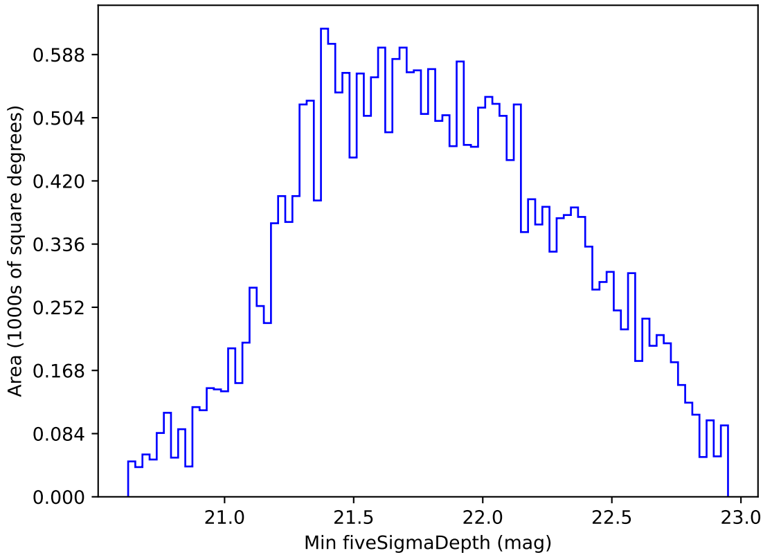
too_elab_r32_d2_ugrizy_v3.4_10yrs All sky i band: Min fiveSigmaDepth
