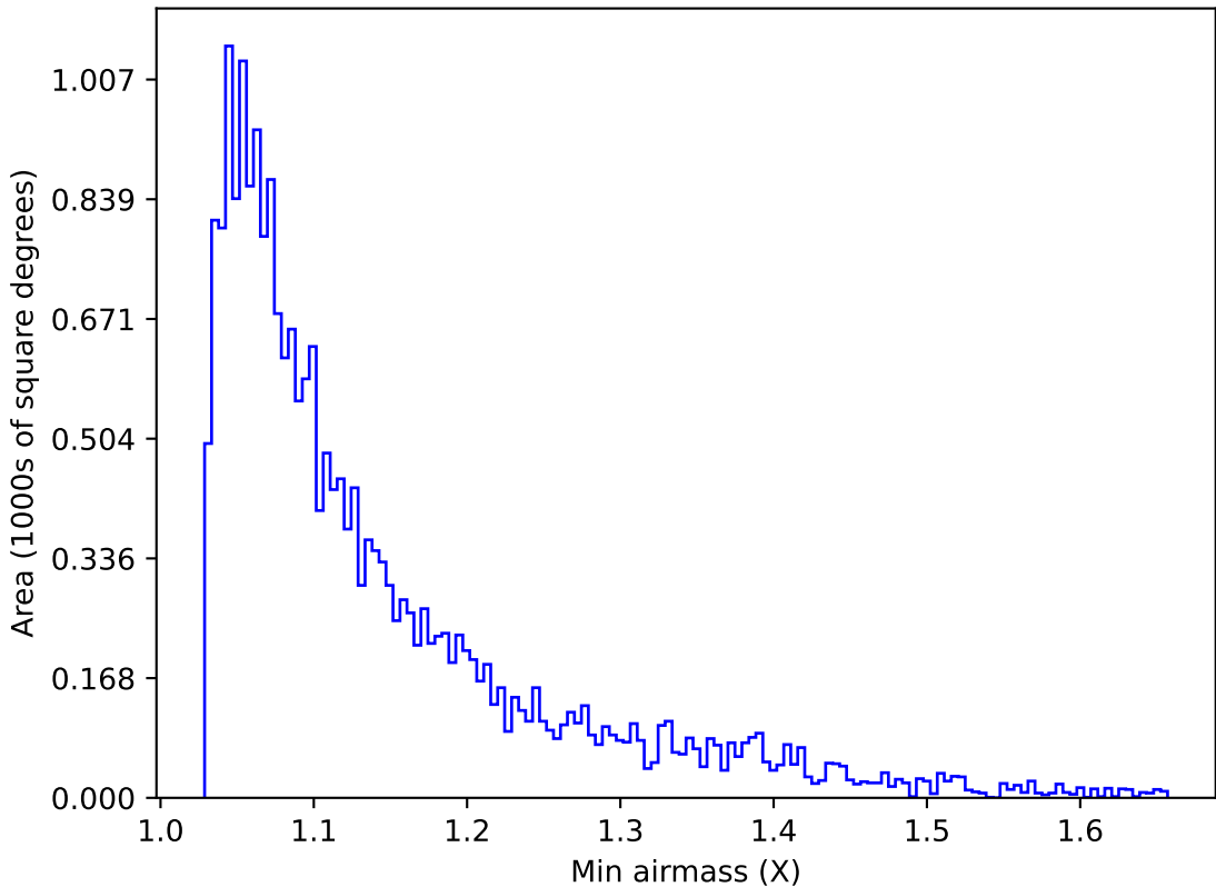
too_elab_r32_d2_ugrizy_v3.4_10yrs Yr 1 u band: Min airmass
