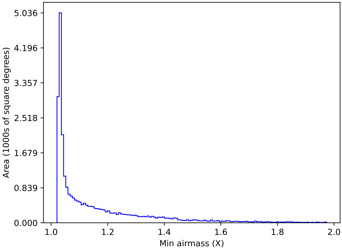
too_elab_r32_d2_ugrizy_v3.4_10yrs Yr 1 all bands: Min airmass
