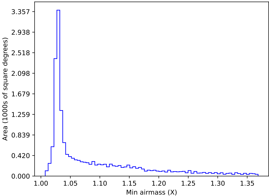
too_elab_r32_d2_ugrizy_v3.4_10yrs WFD z band: Min airmass
