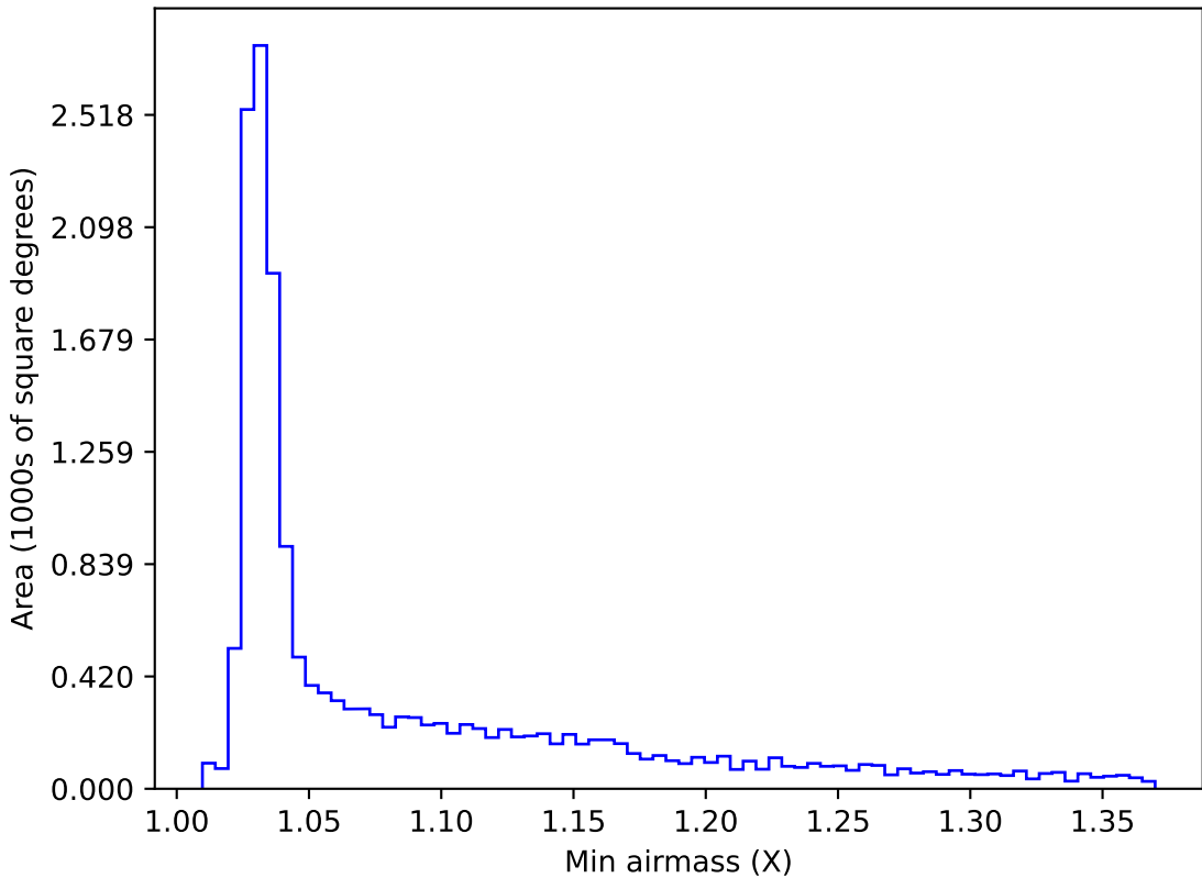
too_elab_r32_d2_ugrizy_v3.4_10yrs WFD y band: Min airmass
