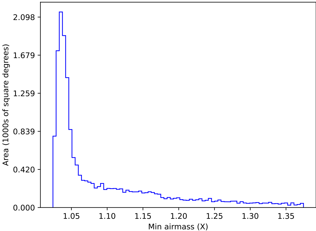
too_elab_r32_d2_ugrizy_v3.4_10yrs WFD u band: Min airmass
