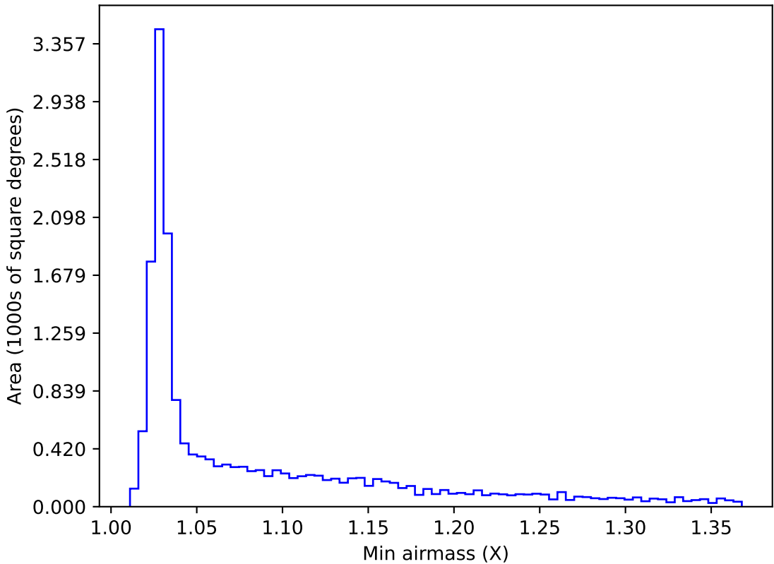
too_elab_r32_d2_ugrizy_v3.4_10yrs WFD i band: Min airmass
