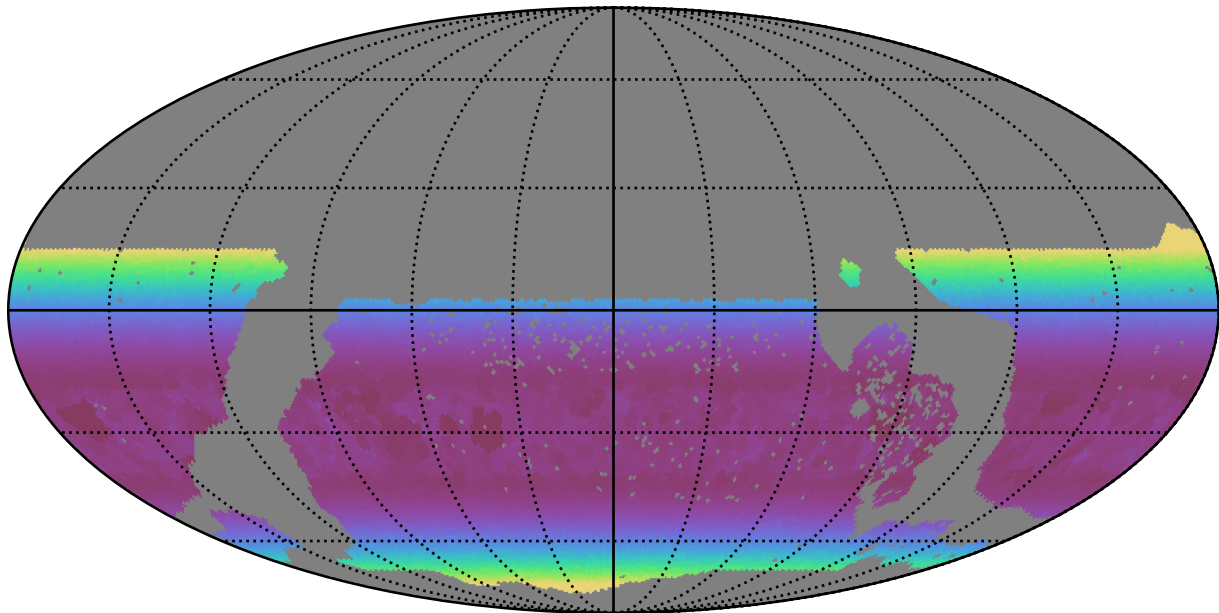
too_elab_r32_d2_ugrizy_v3.4_10yrs WFD g band: Min airmass
