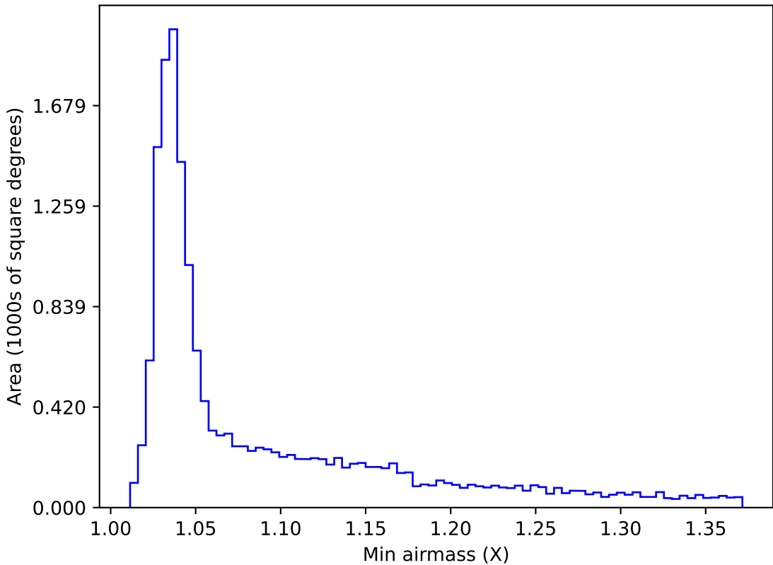
too_elab_r32_d2_ugrizy_v3.4_10yrs WFD g band: Min airmass
