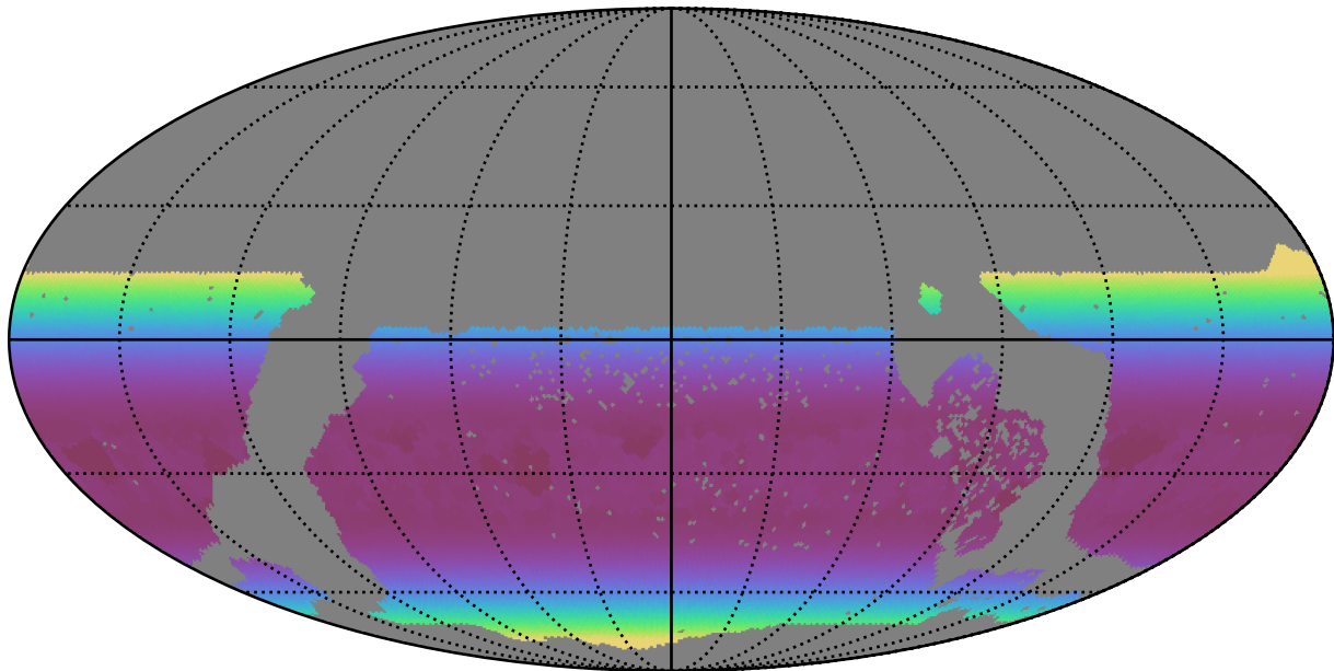
too_elab_r32_d2_ugrizy_v3.4_10yrs WFD all bands: Min airmass
