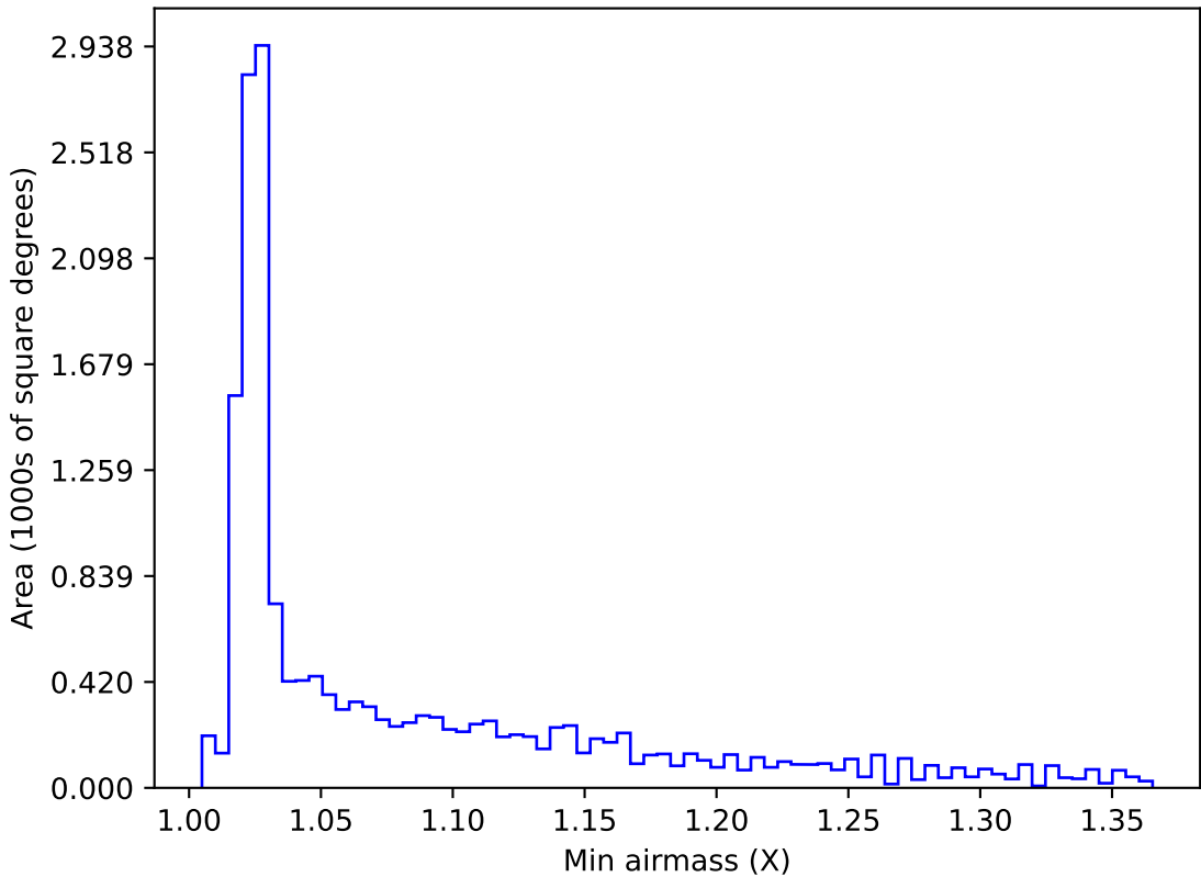
too_elab_r32_d2_ugrizy_v3.4_10yrs WFD all bands: Min airmass
