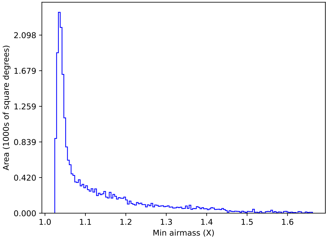
too_elab_r32_d2_ugrizy_v3.4_10yrs All sky u band: Min airmass
