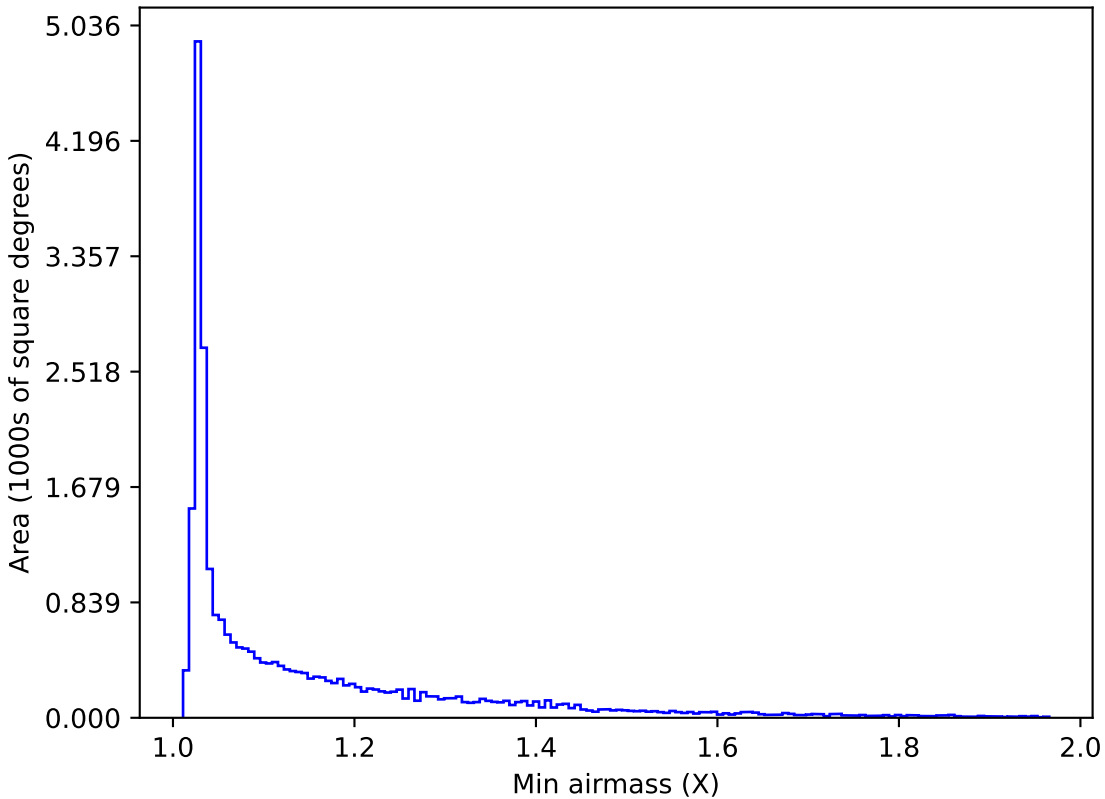
too_elab_r32_d2_ugrizy_v3.4_10yrs All sky i band: Min airmass
