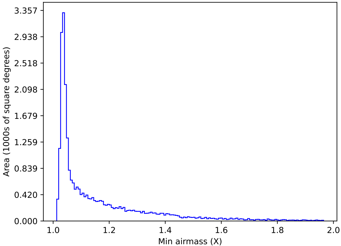
too_elab_r32_d2_ugrizy_v3.4_10yrs All sky g band: Min airmass
