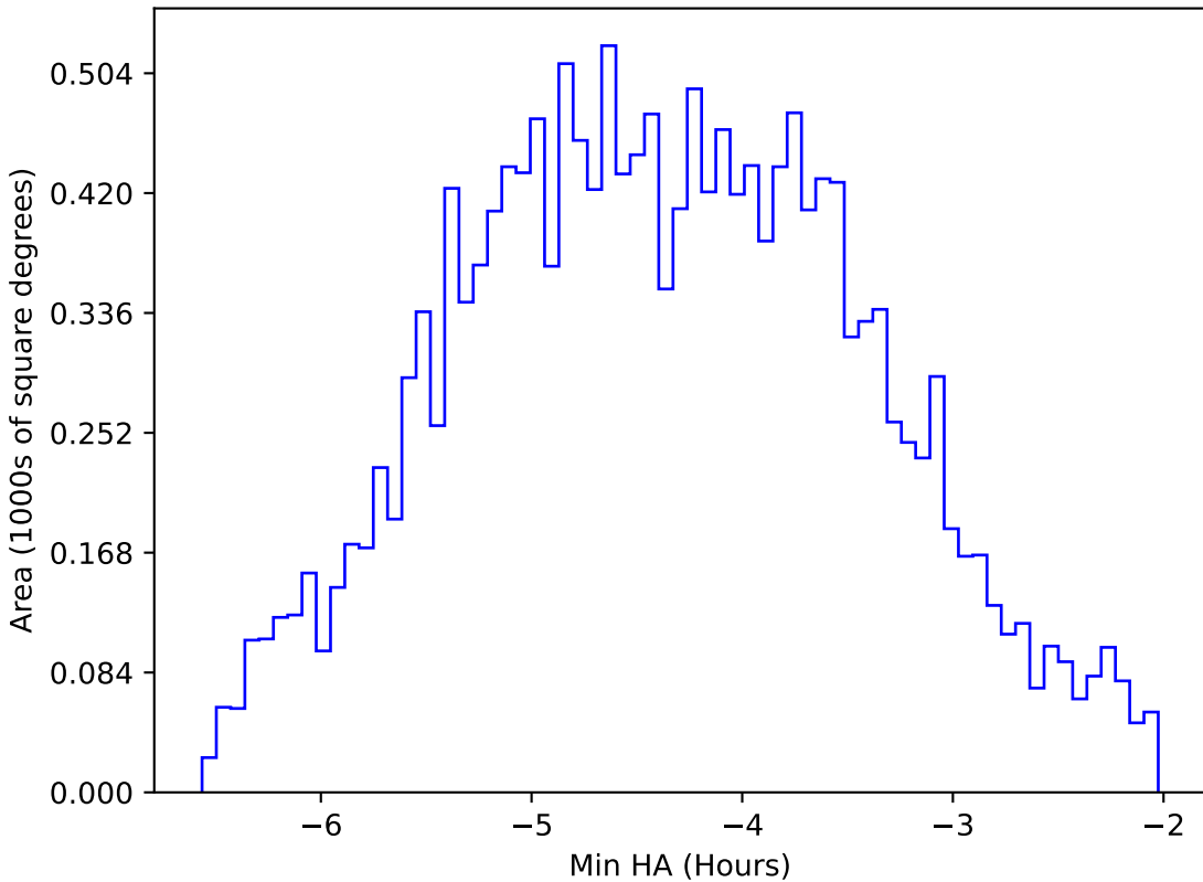
too_elab_r32_d2_ugrizy_v3.4_10yrs WFD z band: Min HA
