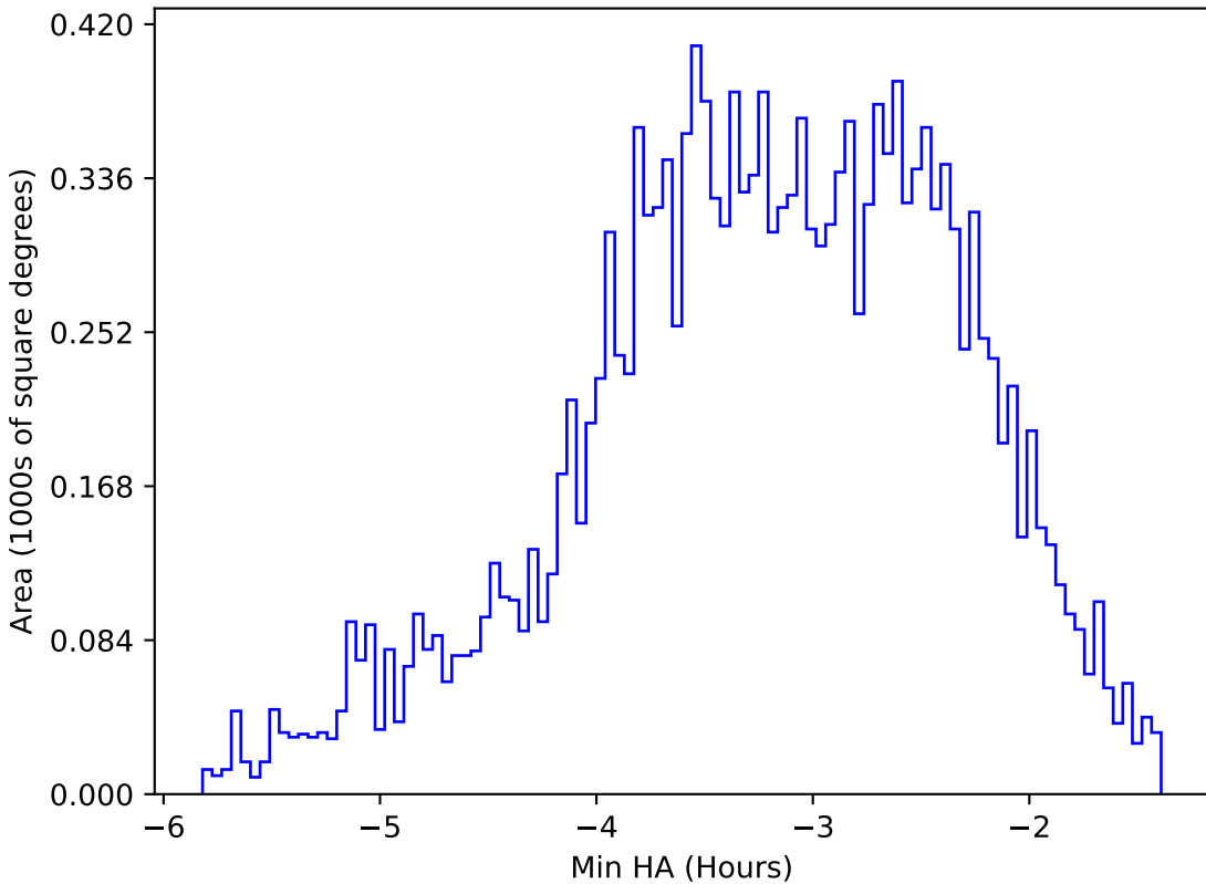
too_elab_r32_d2_ugrizy_v3.4_10yrs WFD u band: Min HA
