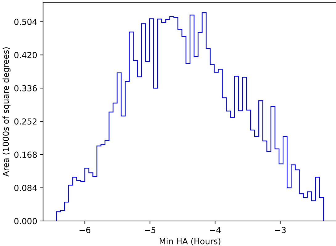
too_elab_r32_d2_ugrizy_v3.4_10yrs WFD r band: Min HA
