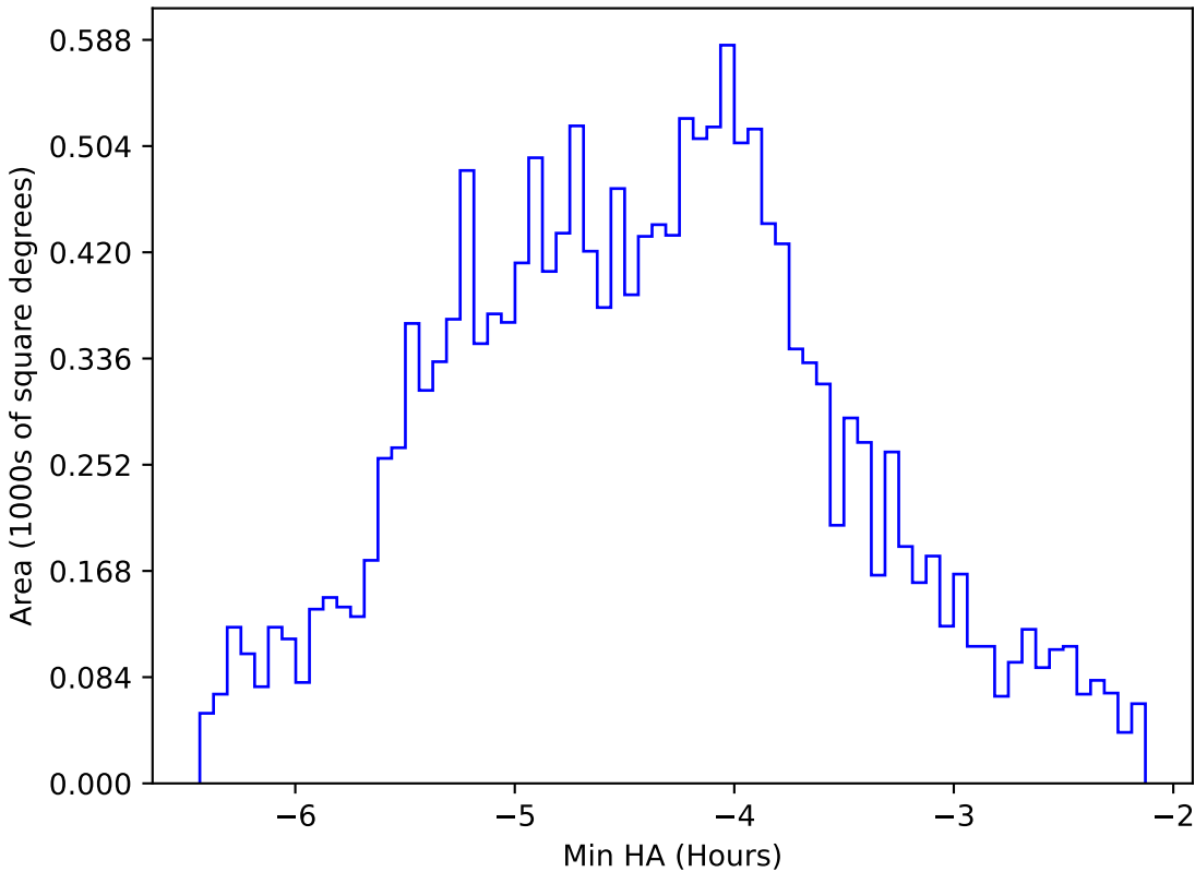
too_elab_r32_d2_ugrizy_v3.4_10yrs WFD i band: Min HA
