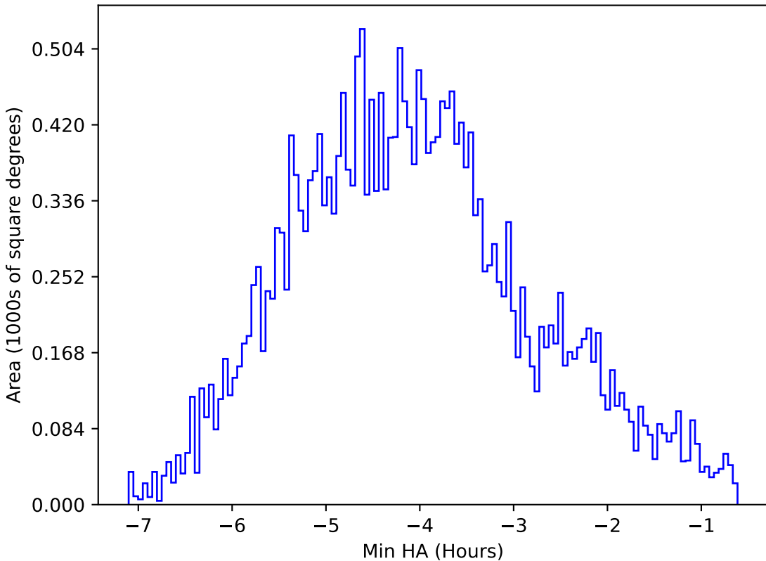
too_elab_r32_d2_ugrizy_v3.4_10yrs All sky z band: Min HA
