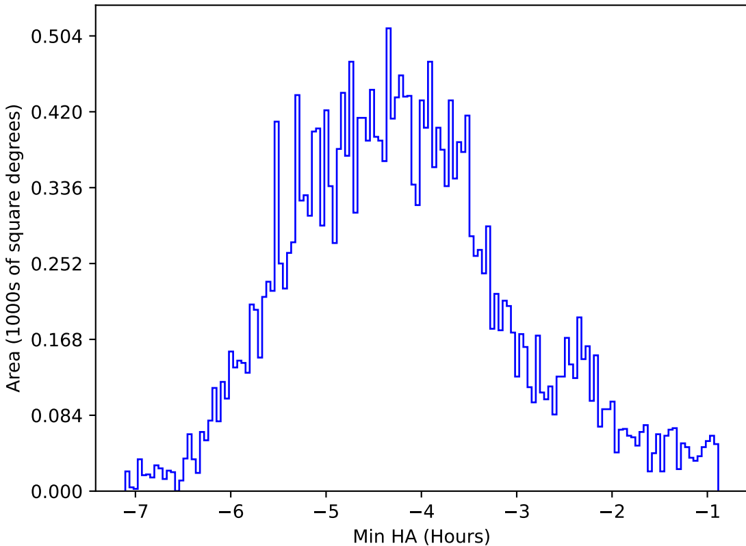
too_elab_r32_d2_ugrizy_v3.4_10yrs All sky r band: Min HA
