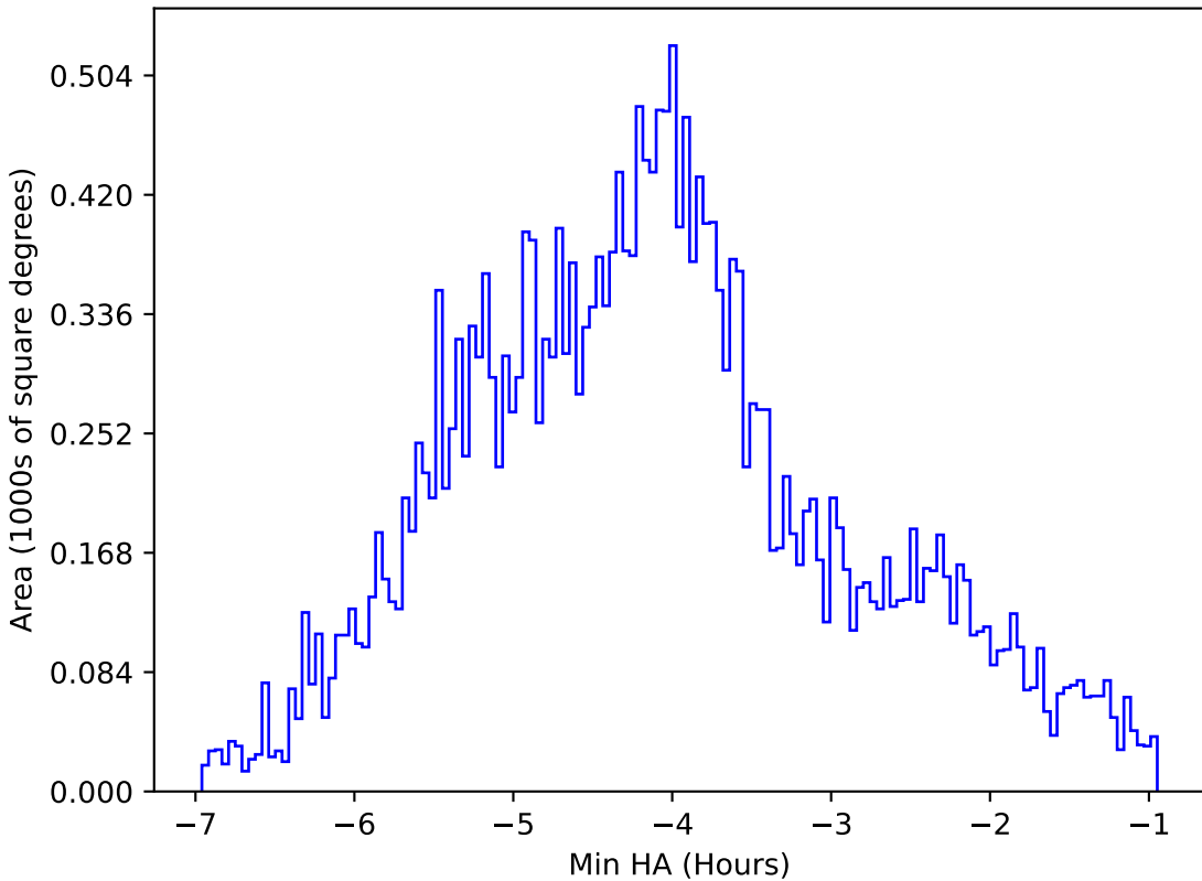
too_elab_r32_d2_ugrizy_v3.4_10yrs All sky i band: Min HA
