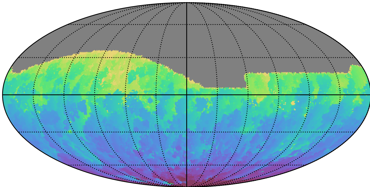
too_elab_r32_d2_ugrizy_v3.4_10yrs All sky g band: Min HA
