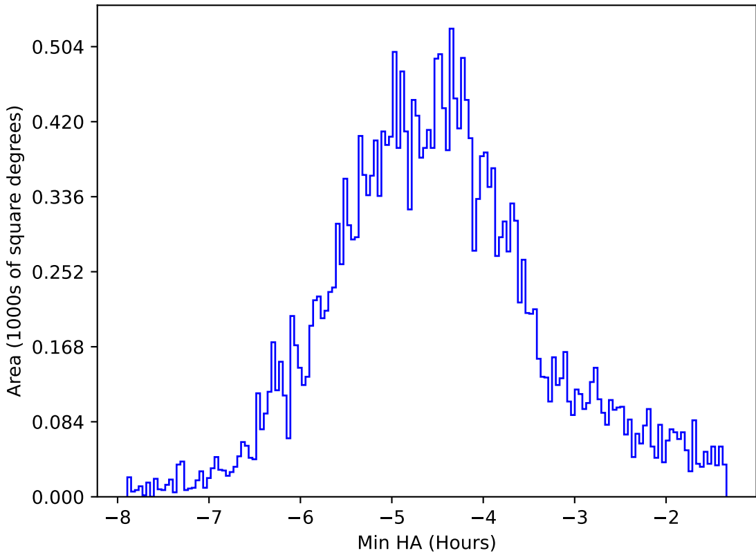
too_elab_r32_d2_ugrizy_v3.4_10yrs All sky all bands: Min HA
