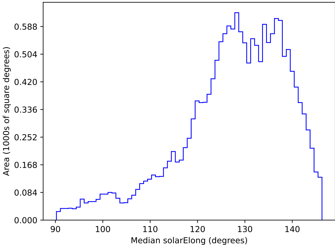
too_elab_r32_d2_ugrizy_v3.4_10yrs WFD z band: Median solarElong
