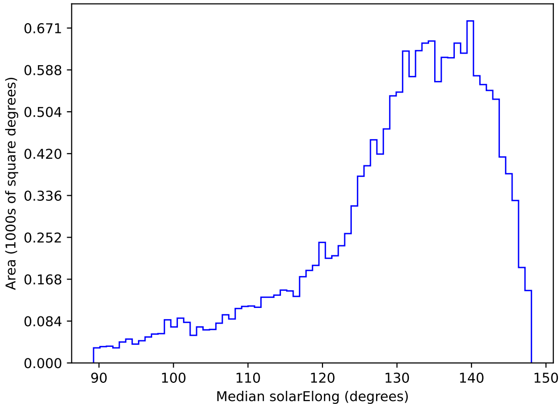
too_elab_r32_d2_ugrizy_v3.4_10yrs WFD y band: Median solarElong
