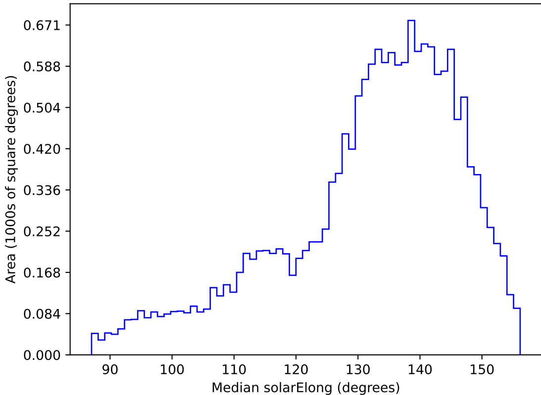
too_elab_r32_d2_ugrizy_v3.4_10yrs WFD u band: Median solarElong
