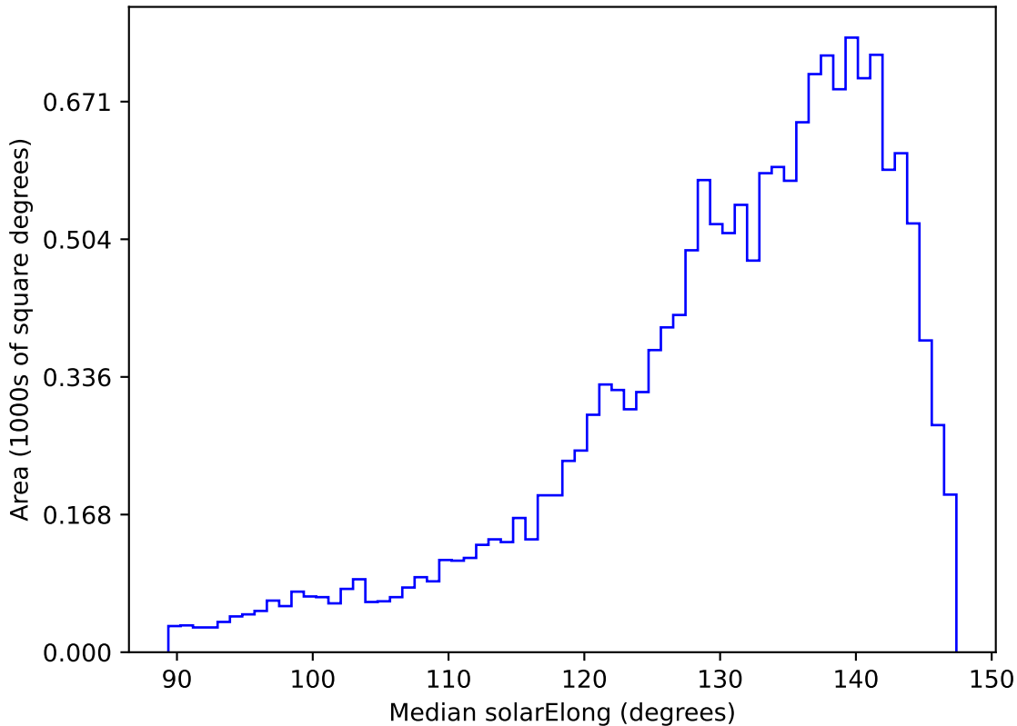
too_elab_r32_d2_ugrizy_v3.4_10yrs WFD r band: Median solarElong
