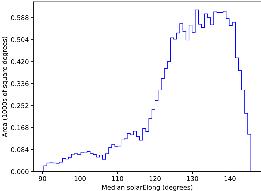
too_elab_r32_d2_ugrizy_v3.4_10yrs WFD i band: Median solarElong
