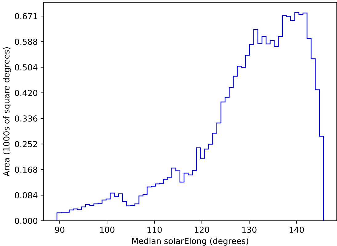
too_elab_r32_d2_ugrizy_v3.4_10yrs WFD all bands: Median solarElong
