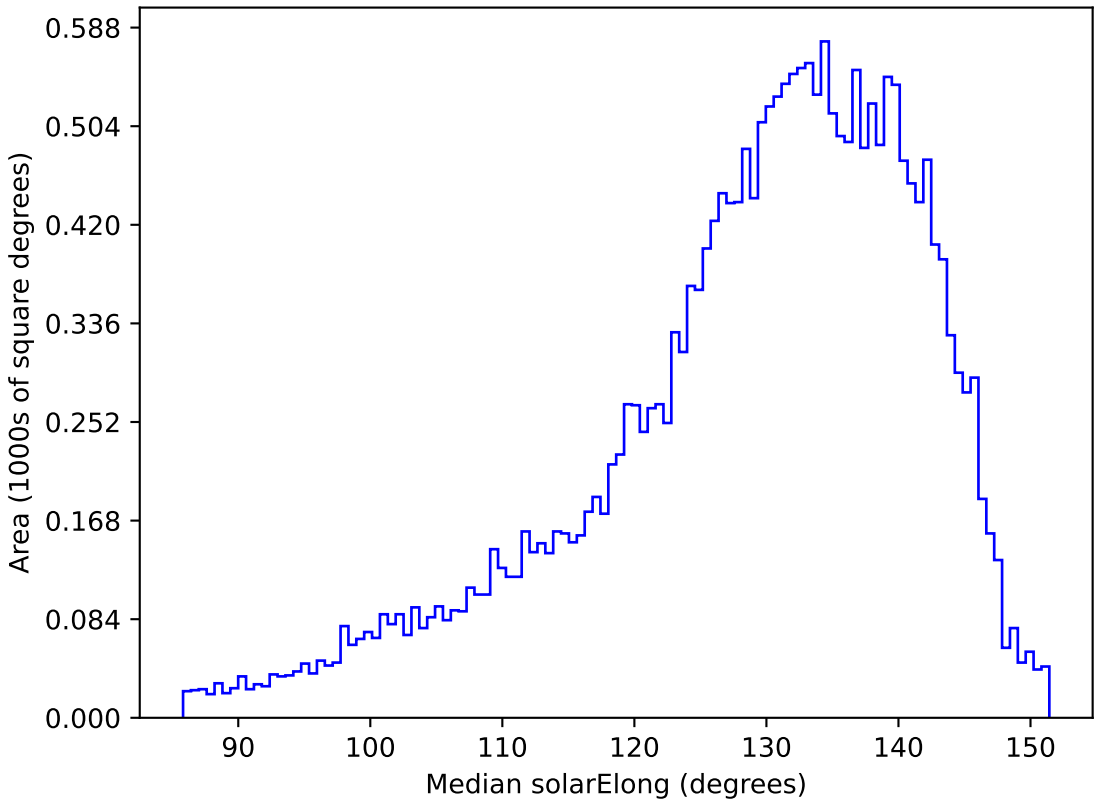
too_elab_r32_d2_ugrizyv3.4_10yrs All sky y band: Median solarElong
