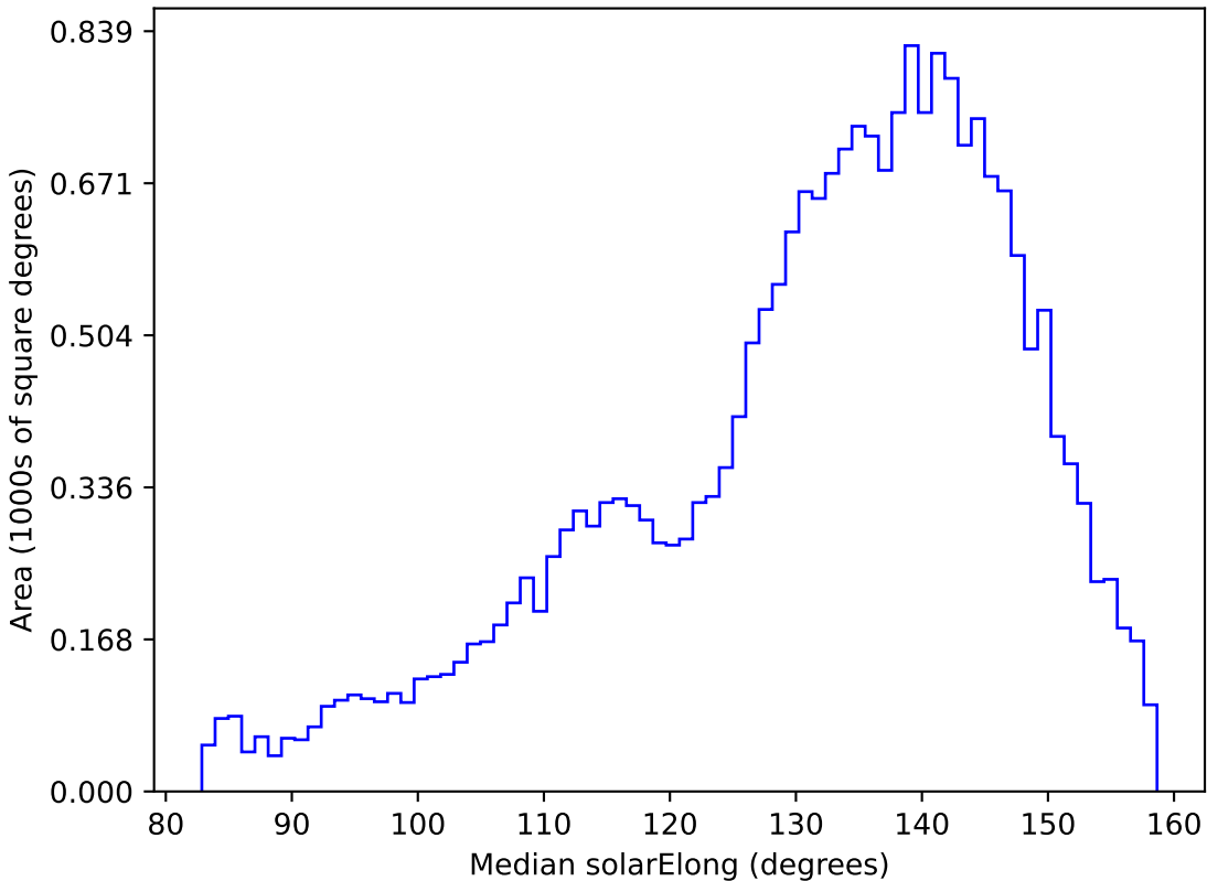
too_elab_r32_d2_ugrizy_v3.4_10yrs All sky u band: Median solarElong
