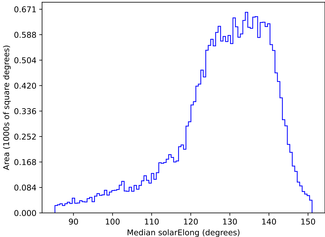
too_elab_r32_d2_ugrizy_v3.4_10yrs All sky i band: Median solarElong
