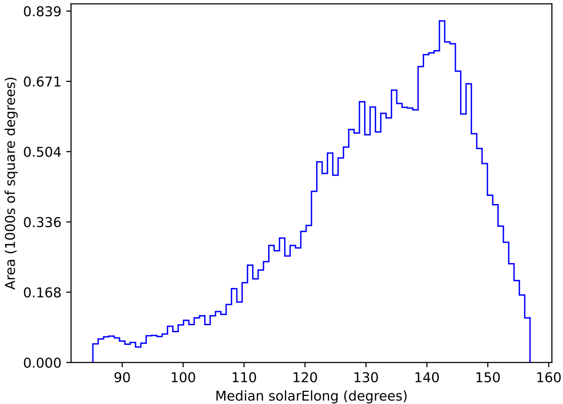
too_elab_r32_d2_ugrizy_v3.4_10yrs All sky g band: Median solarElong
