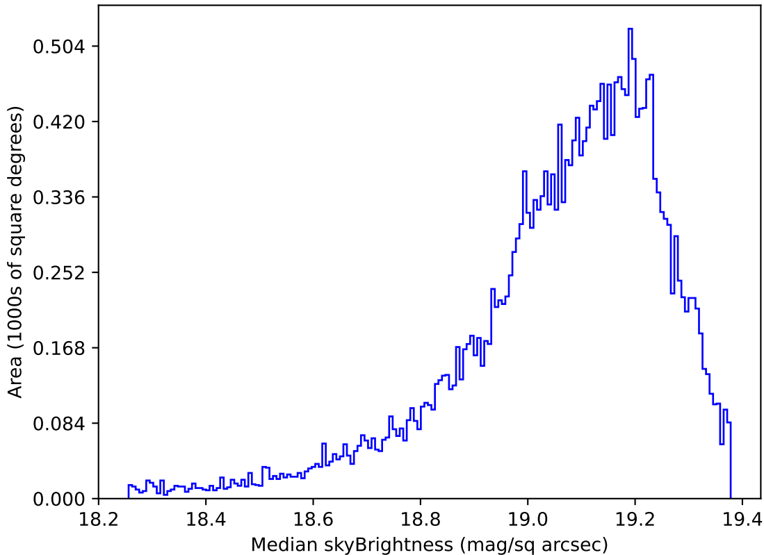
too_elab_r32_d2_ugrizy_v3.4_10yrs Yr 1 z band: Median skyBrightness
