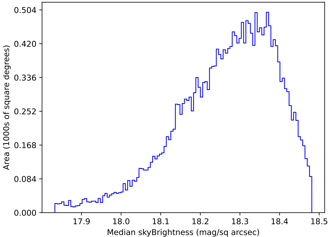
too_elab_r32_d2_ugrizy_v3.4_10yrs Yr 1 y band: Median skyBrightness
