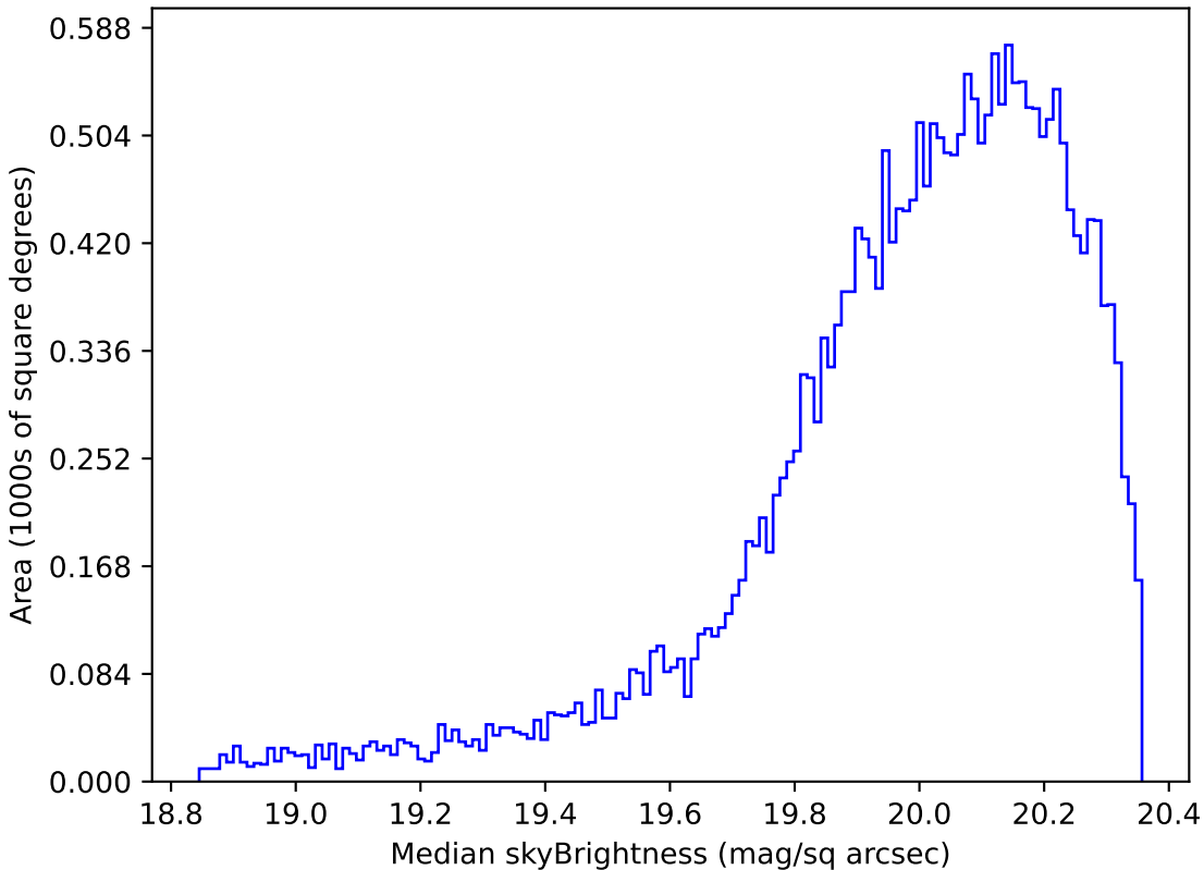
too_elab_r32_d2_ugrizy_v3.4_10yrs Yr 1 i band: Median skyBrightness
